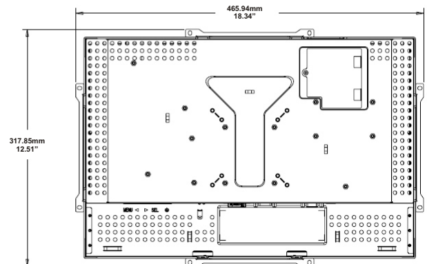
REAR MOUNT WITH BRACKETS, HORIZONTAL & VERTICAL
