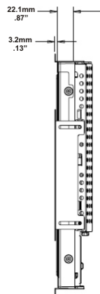
MOUNTING BRACKET ADJUSTMENT RANGE
